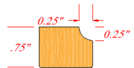
L - 1/4" Cove
