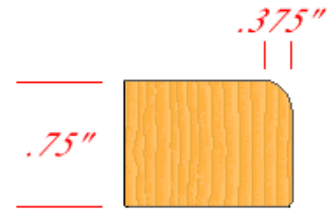
C - 3/8" Round
