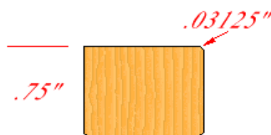
H - Eased
