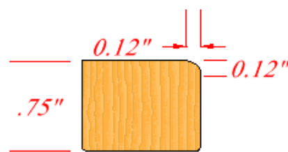
K - 1/8" Round
